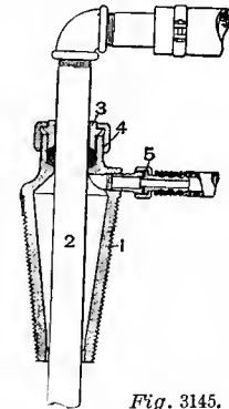
Fig. 3145. Section of Transfer-plug.
